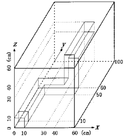
Figure 8. Sketch of Problem 3, shield with dog leg void duct
