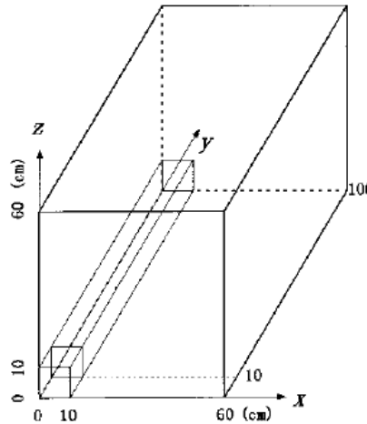
Figure 4. Sketch of Problem 2, shield with void duct
