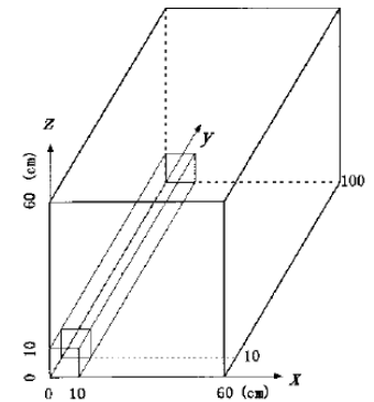
Figure 4. Sketch of Problem 2, shield with void duct
