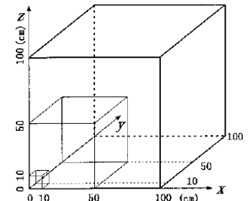
Figure 2. Sketch of Problem 1, shield with square void
