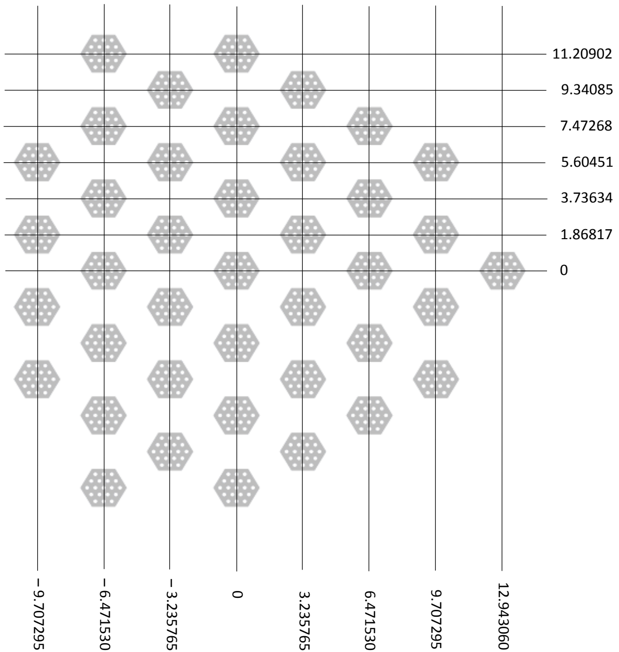
Plane View of the Array of 40 NRX-A4 Elements
